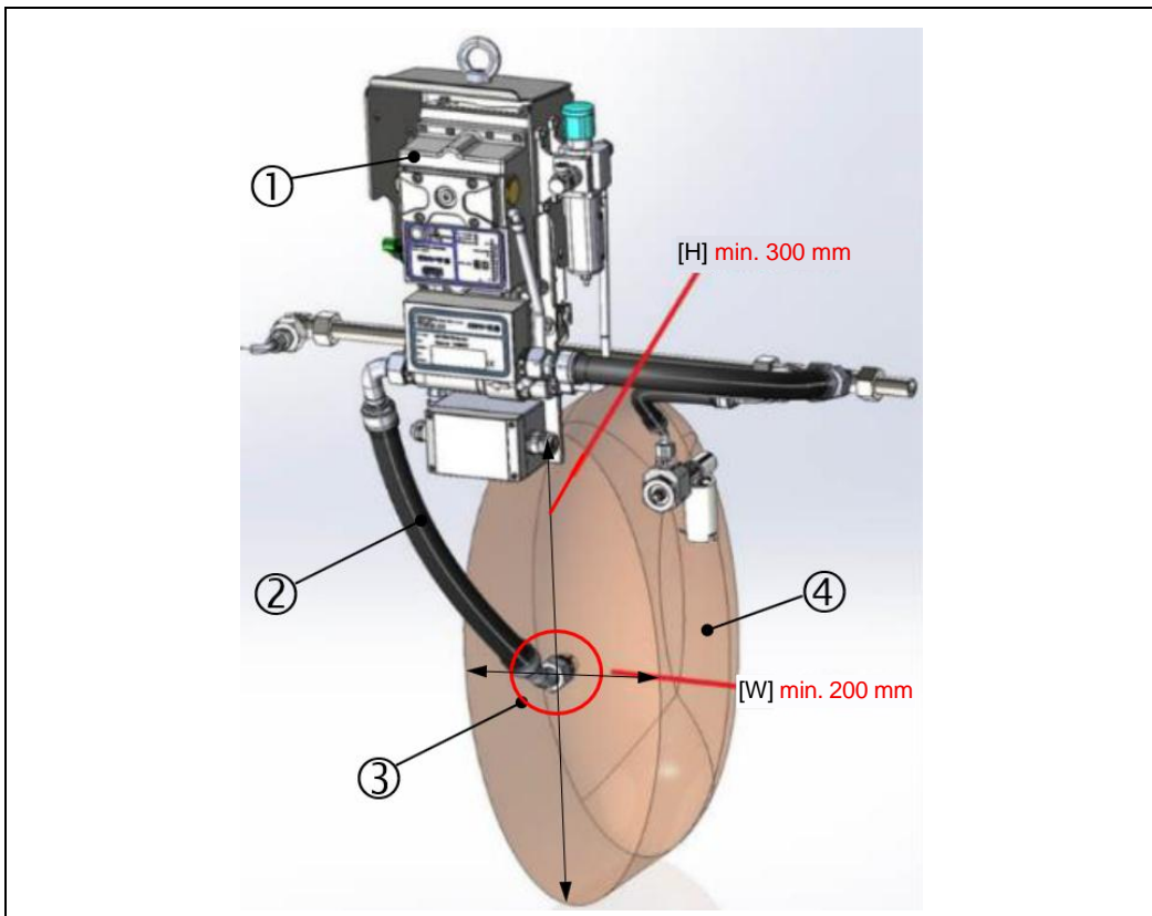
Fig.: 35 : Position of the recirculation line on the VN2020
