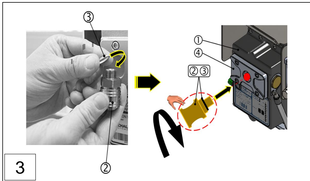
1: Measuring head 2: Quick-release coupling 3: Sealing ring 4: Inspection cover
