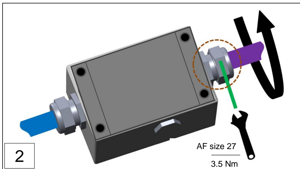
Fig.: 50 : Connecting the Remote Indicator II to terminal box (example inst.; install. steps 1-2)
