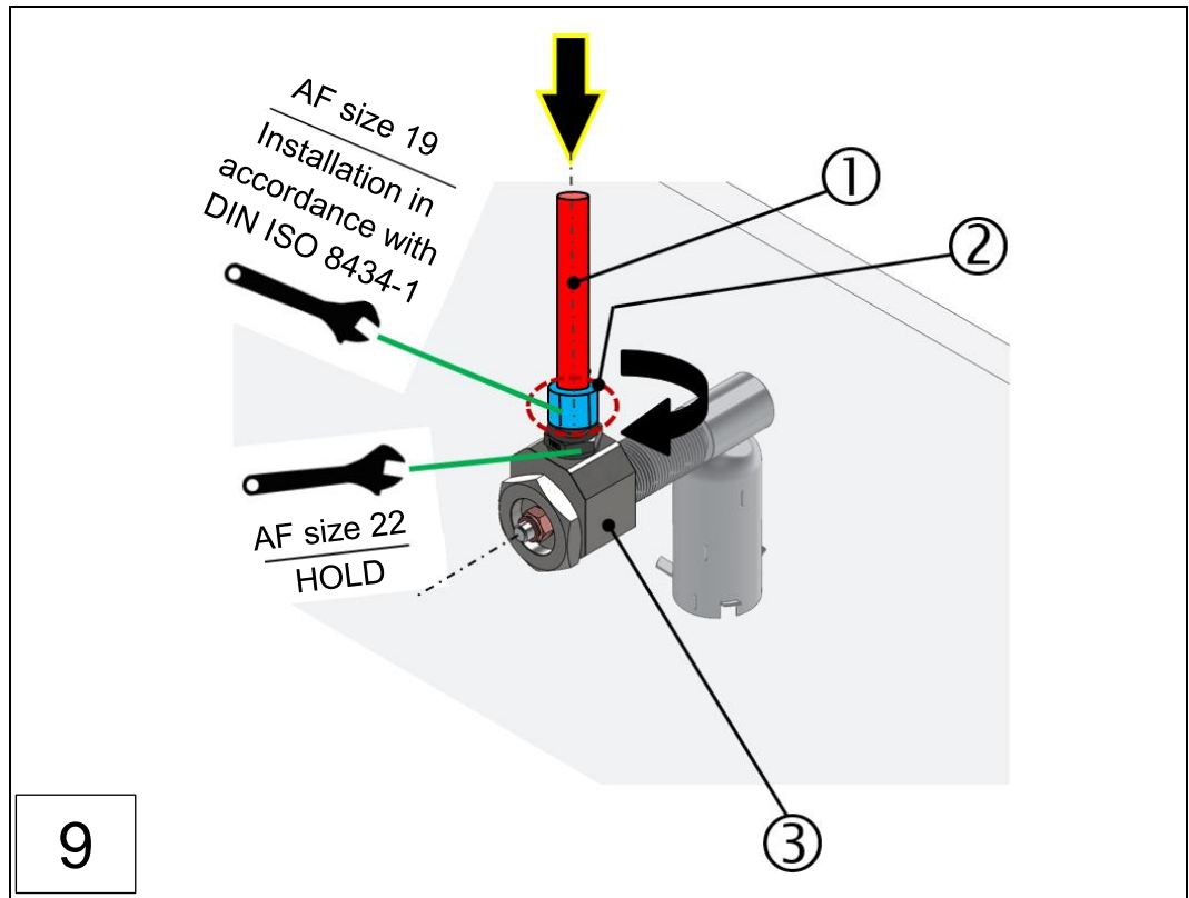
Fig.: 29 : Installing the engine wall connection for the VN200 (installation steps 1-9)
