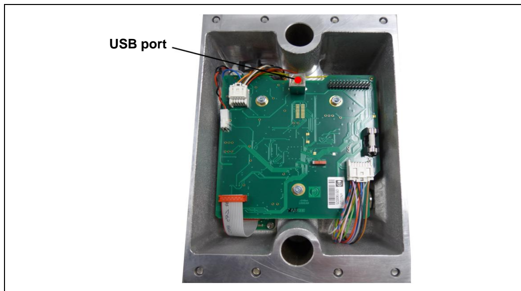
Fig.: 65 : Measuring head for VN2020, rear view, USB port
