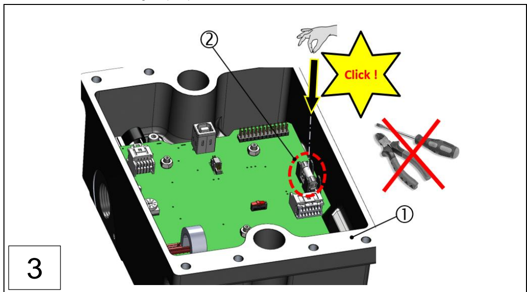
Fig.: 85 : Replacing the fuse on the VN2020 measuring head (steps 1-3)
