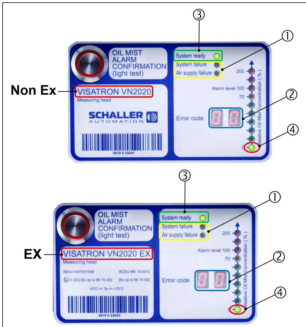
Fig.: 56 : “System ready” indicator on the VN2020/VN2020 EX measuring head
