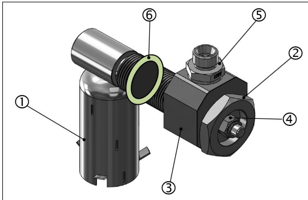
Fig.: 27 : Engine wall connection (EWC)
