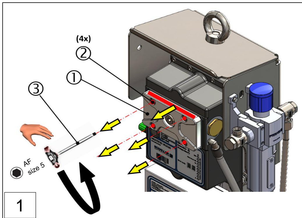
1: Inspection cover
