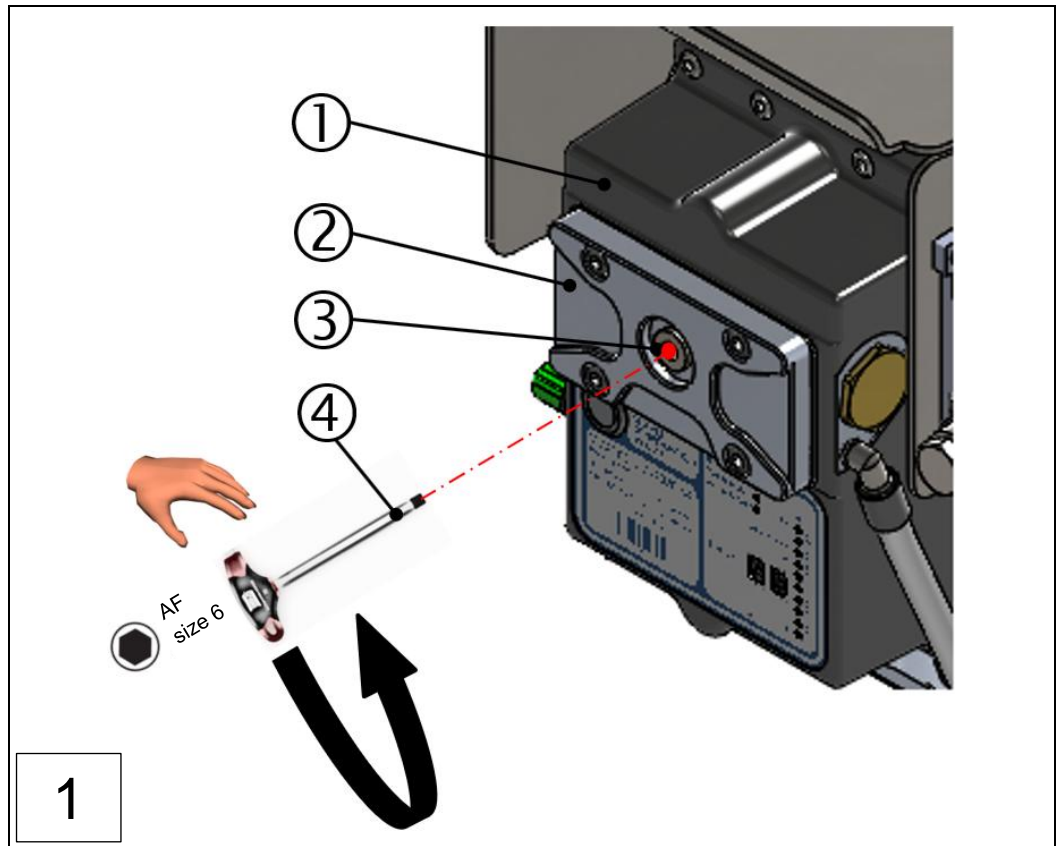
1: Measuring head 2: Inspection cover 3: Screw plug 4: Allen key, size 6/torque spanner for 15 Nm
