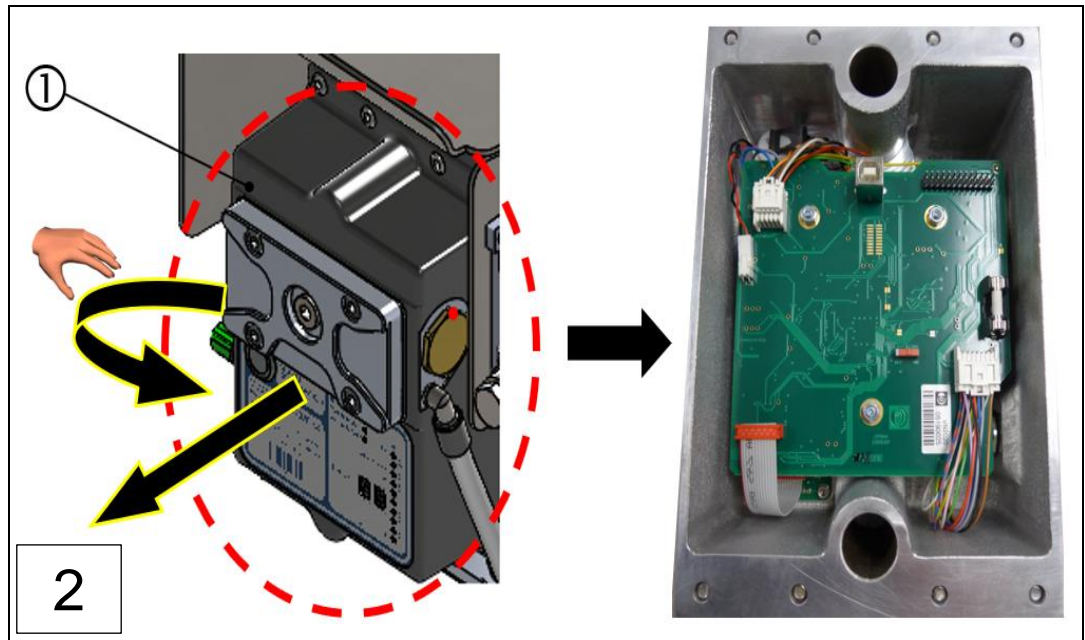
Fig.: 66 : Removing the VN2020 measuring head (installation steps 1-2)
