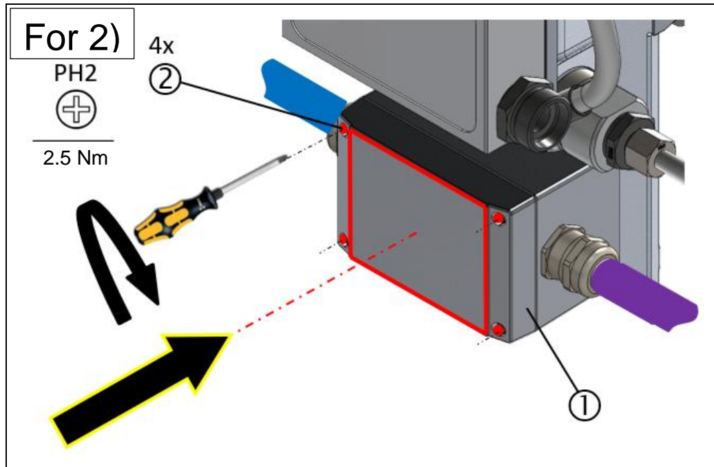
Fig.: 89 : Replacing the VN200 terminal box (installation steps 1-8)
