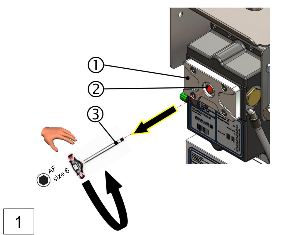
1: Inspection cover 3: Allen key, size 6
