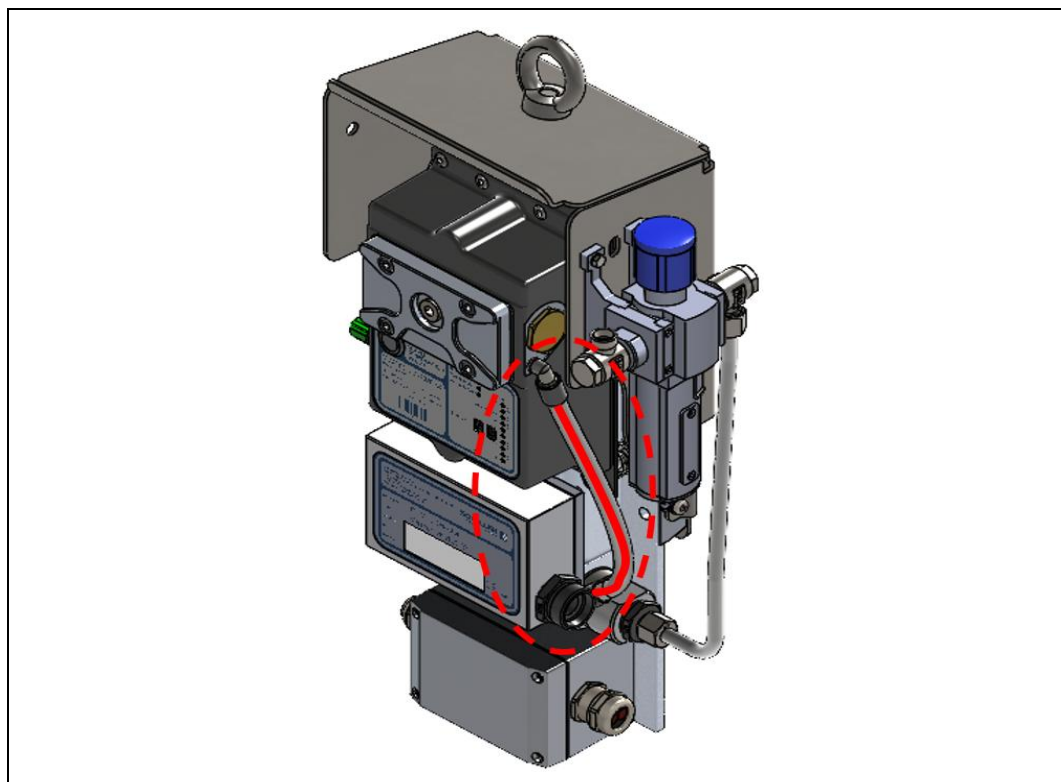
Fig.: 92 : Connecting hose, VN2020 oil mist detector
