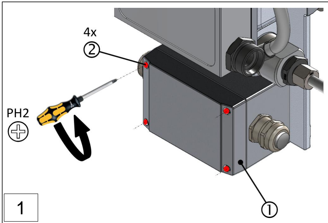
1: Cover, VN2020 terminal box
