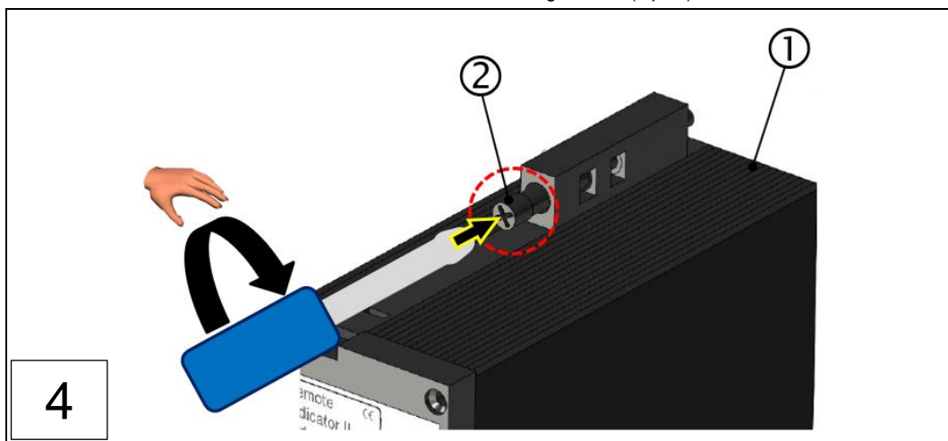
4 Fig.: 40 : Installing Remote Indicator II (installation steps 1-4) 1: Remote Indicator II 2: Fixing screws (2 pcs.)
