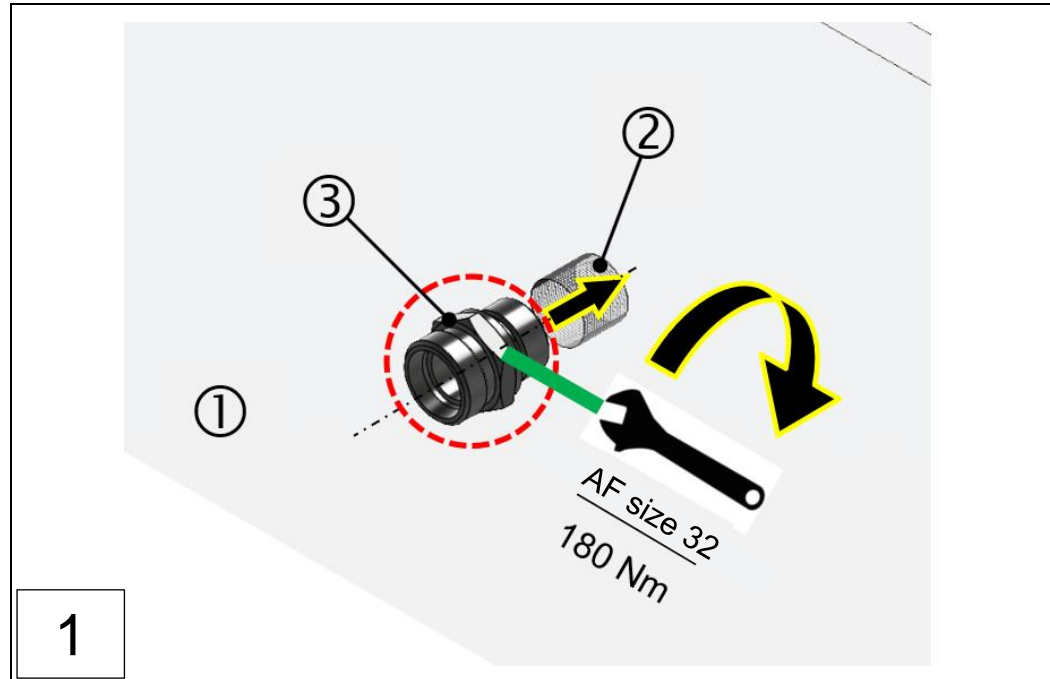
1: Engine wall 2: Screw-in thread on engine wall 3: Straight screw-in socket L22
