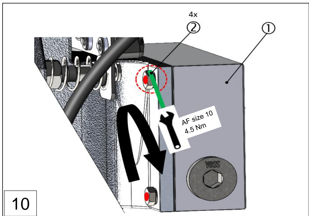
1: Connecting box
