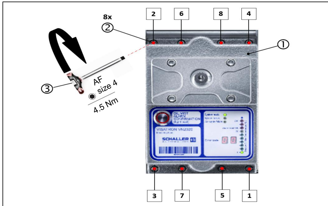
Fig.: 68 : Installing the VN2020 measuring head
