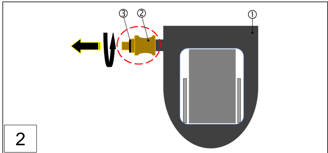
1: U-tube manometer (accessory) 2: Quick-release coupling 3: Sealing ring
