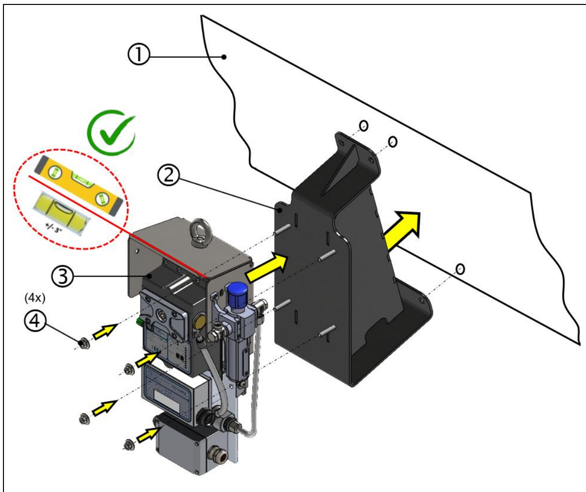
Fig.: 24 : Installing VN2020 with bracket and protective cover
