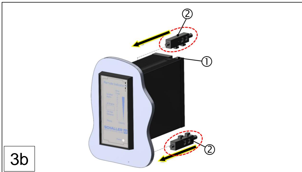
3b 1: Remote Indicator II 2: Retaining bracket (2 pcs.)
