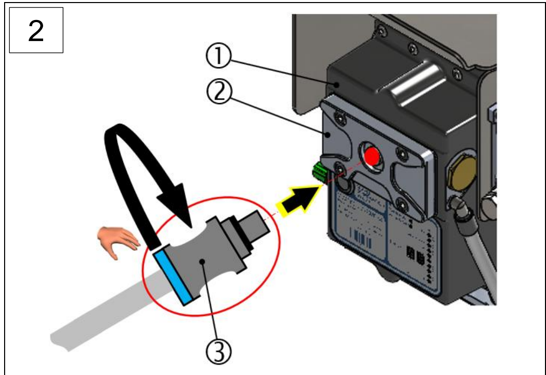
1: Measuring head 2: Inspection cover 3: Push-in fitting with flexible hose ▶ (3) is the same as 4 and 5 in Figure 79 in this section. ▶ (3) is screwed hand-tight into the inspection cover (2).
