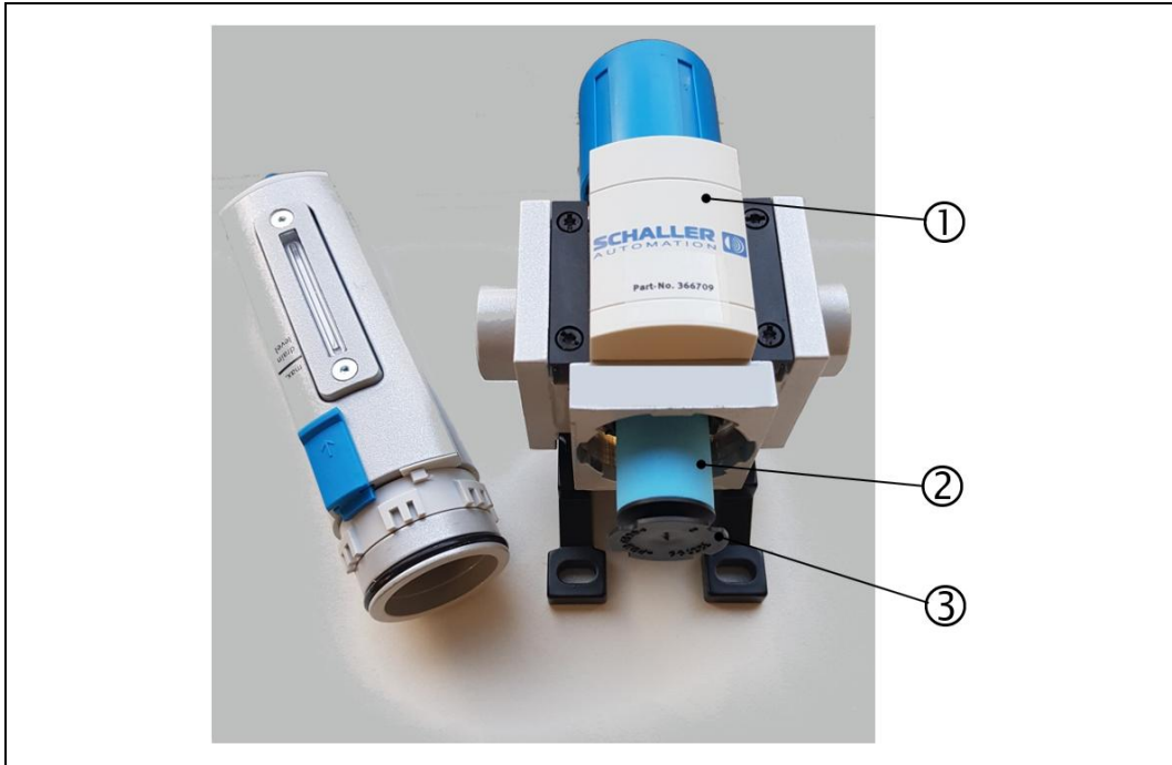
Fig.: 77 : Replacing the air filter element on the pressure regulator unit
