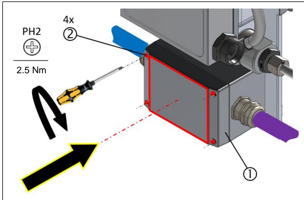
Fig.: 53 : Closing the terminal box for VN2020
