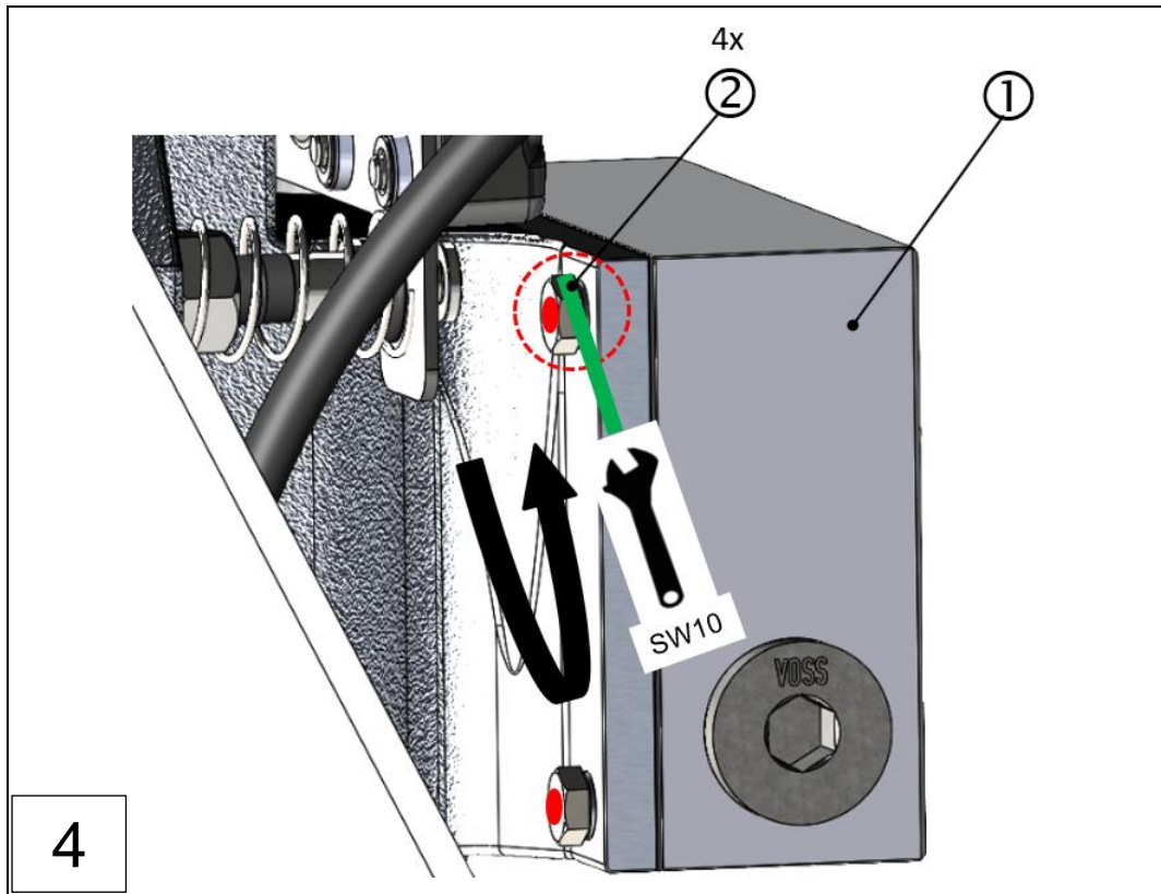
1: Anschlusskasten VN2020 EX-H2 "
