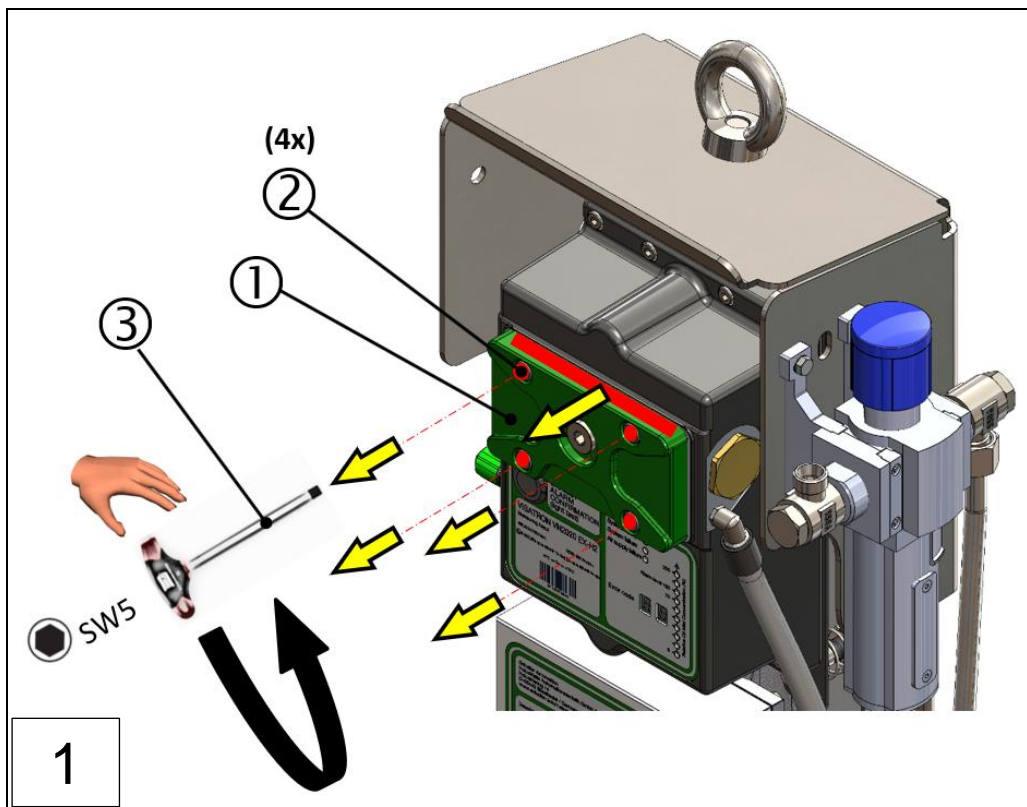
1: Kontrolldeckel VN2020 EX-H2
