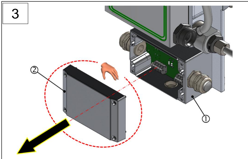
1: Klemmenkasten VN2020 EX-H2
