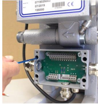
Figure 131: remove screws
