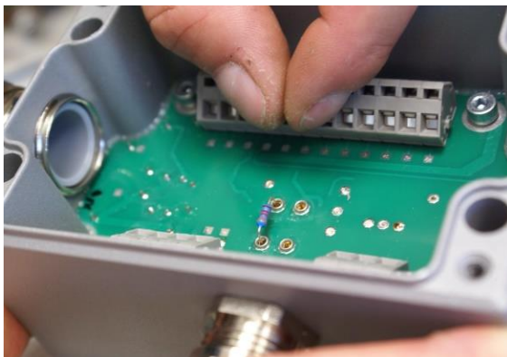
Figure 46: Insert resistor
