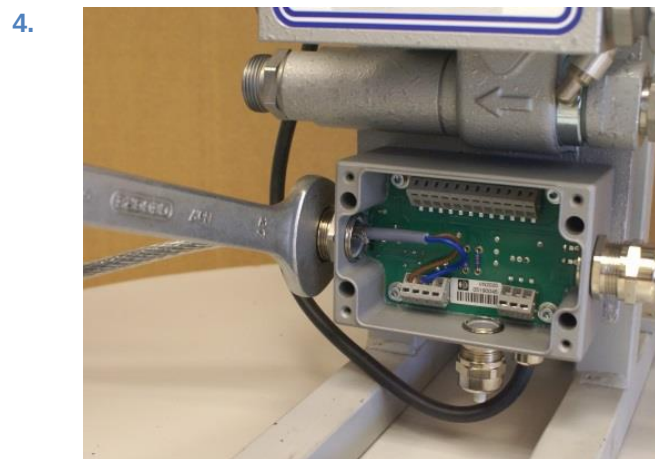
Figure 127: loosen cable glands
