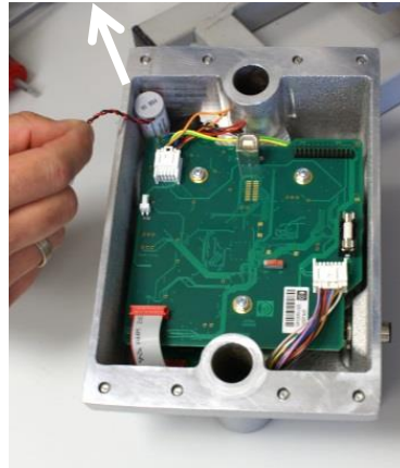
Figure 113: remove battery
