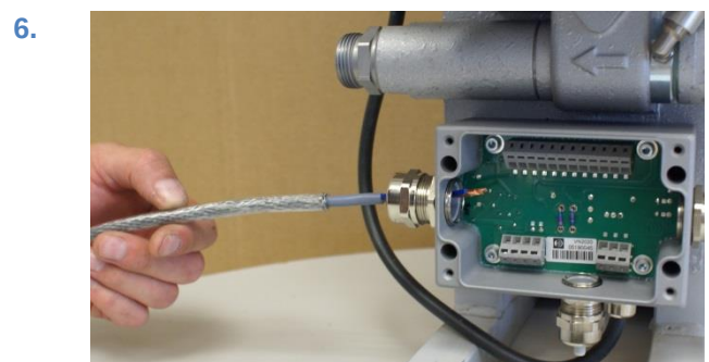
Figure 129: pull out cable
