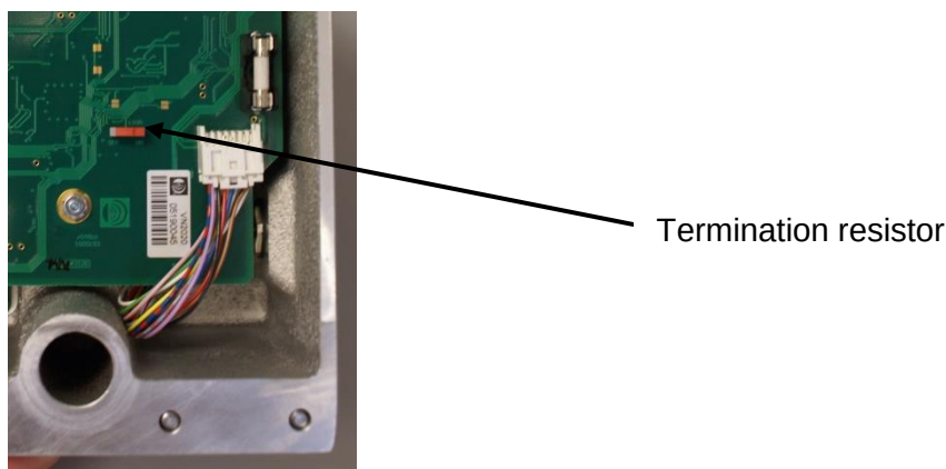
Figure 52: Switchable termination resistor
