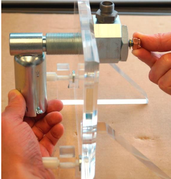
Figure 17: Align the suction funnel
